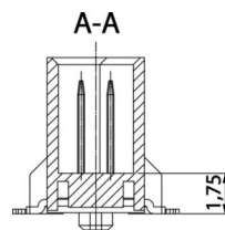
32 Pins
